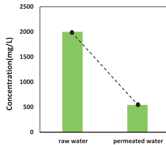
Figure 1: Concentration of Mg^{2+} in raw water and permeated water
