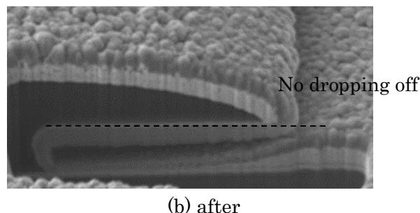
Fig.1. SEM images of resist profiles of before and after improving.
