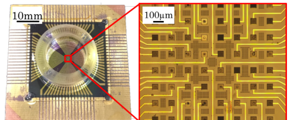
Fig.1 Photographs of the fabricated device.
